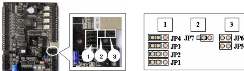
Figure: Jumper Switch location and setting for RS_422 communication
