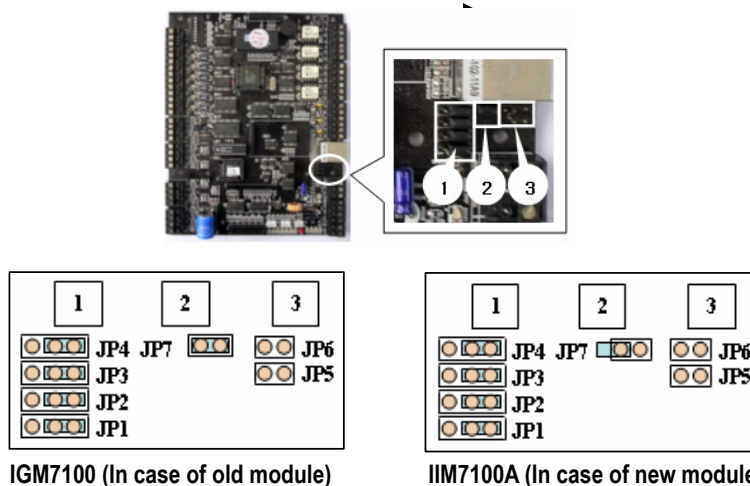
Figure: Jumper Switch location and setting for LAN (TCP/IP module) communication
