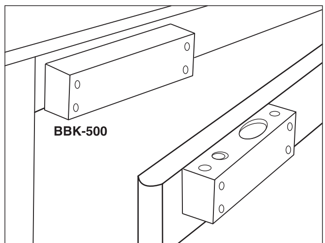
Bracket Installation Diagram
